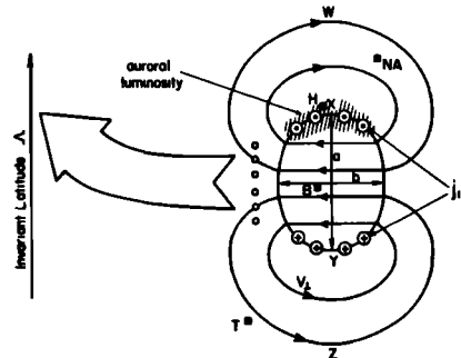
Fig. 4. Schematic snapshot of flows, V_1 , field, aligned currents, j_{||} , optical arcs and isolated, newly-connected flux tube (axes a and b) for initial, westward motion over observing stations (see fig. 1). The broad arrow shows the subsequent path of the event. The full potential is applied between X and Y, that between W and Z is zero.
