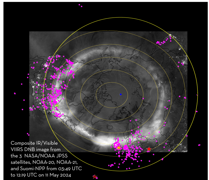
Figure 6. Area-combined auroral samples (mauve points) mapped onto a composite Near-IR/Visible DNB image for the Northern Hemisphere auroral oval during the 10–11 May 2024 Event. This composite is made from images from 3 satellites (unlike Figure 3 which is made from just one): the NOAA/NASA JPSS satellites, NOAA-20, NOAA-21, and Suomi-NPP. The mauve dots are locations from which aurora was reported from the ground on 10 and 11 May 2024 and the orange contours are QD geomagnetic latitudes, \Lambda_M , of [40^\circ:10^\circ:80^\circ] for that date. The yellow circle is at geographic latitude \Lambda_G = 35^\circ and enables comparison with Figure 3. The coloured stars are the locations from where the images shown in Figure 7 were recorded. Image courtesy the VIIRS Imagery and Visualization Team, CIRA, Colorado State University, USA.
