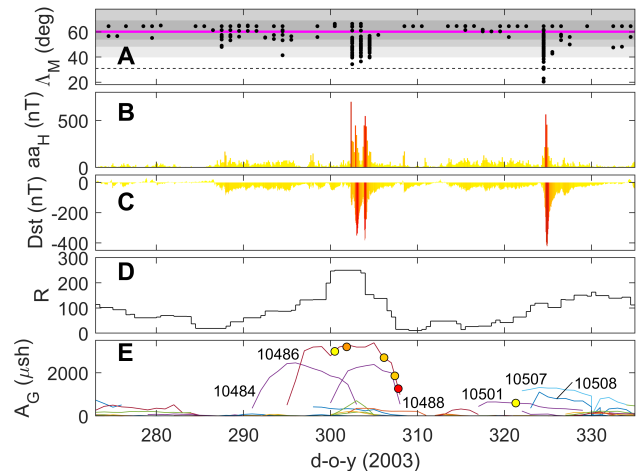
Figure 17. Analysis of the “Halloween” events of October/November 2003, followed by the 20 November 2003 extreme auroral event. The format is the same as Figure 2. In part E the numbers are the numbers of the sunspot groups labelled in Figure 18 and yellow dots denote the occurrence of an M-class flare in that sunspot group and orange and red points denote X-class flares, the red point being the largest flare ever recorded. The horizontal dashed line in A is the 31^\circ threshold of \Lambda_M used in this paper to define extreme auroral events.
