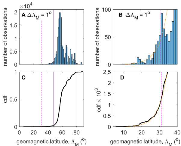
Figure 11. Distributions of the number of area-combined samples, N with QD geomagnetic latitude, \Lambda_M . A is a histogram of the full distribution in bins of \Lambda_M that are \Delta\Lambda_M = 1^\circ degree wide. B Detail of the low latitude tail of the distribution shown in A with the orange line being the best-fit exponential rise of the distribution at \Lambda_M < 45^\circ which is given by ae^{(b\Lambda_M)} where a = 0.058 and b = 0.216 . Part C is the cumulative distribution function (CDF) corresponding to A : the solid vertical mauve lines are the 2\sigma points of the distribution. Part D is the CDF corresponding to B and the orange line again shows the best exponential fit. The vertical dashed line in all plots is at \Lambda_M = 31^\circ and marks the point where the distribution departs from the exponential. This is taken in this paper to be the threshold latitude for an extreme event. The CDF at this threshold shows that below this latitude are just 0.126% of auroral sightings. The median auroral latitude is 57.023^\circ , the 1\sigma range is 54.03 to 68.01^\circ , the 2\sigma range is 47.63 to 77.76^\circ and the 3\sigma range is 31.36 to 86.55^\circ .
