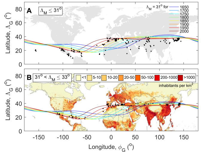
Figure 12. Maps of A locations of observations at geomagnetic QD latitudes below 31^\circ (black points) and B of observations at low latitudes that do not quite meet the \Lambda_M \leq 31^\circ criterion, being at 31 < \Lambda_M \leq 33^\circ . The coloured contours on both panels are of \Lambda_M = 31^\circ for the years of [1650:2000]. The map in Panel B shows the global population density (in individuals per \text{km}^2 ) in modern times (2022) (Mathieu & Rodés-Guirao 2022).
