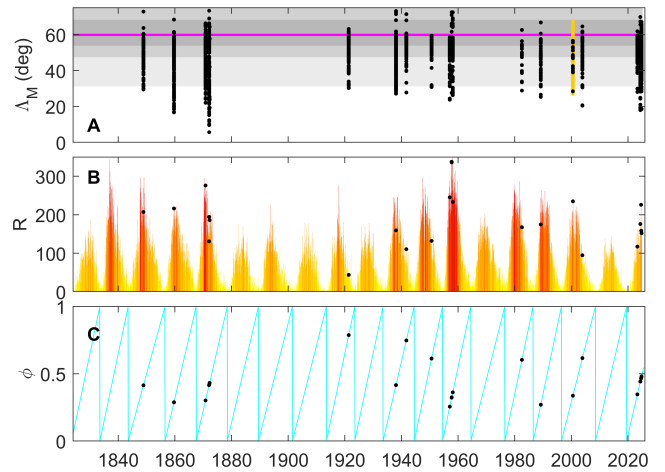
Figure 14. Analysis of extreme auroral events in which aurora extends to geomagnetic latitudes below the \Lambda_M = 31^\circ threshold (that is defined in Figure 11) for January 1820 to June 2024. A the black points show the \Lambda_M of area-combined samples on days classed as extreme events. The bars of different shades of grey and the mauve line give the distribution and mean of \Lambda_M for all samples in the database, using the same format as in Figure 13. The orange bar for the ‘Bastille Day’ event of 14 July 2000 gives the range of \Lambda_M derived from global auroral images from UV imager on the Polar spacecraft which is used because cloud cover and the timing of the event combined to give fewer ground-based observations of aurora in this event at the lowest \Lambda_M . B Carrington Rotation means of sunspot number, R , in the same format as Figure 8B. The black points are the values for the CR containing the extreme event. C The solar cycle phase variation, \phi , with the black points marking the extreme events.
