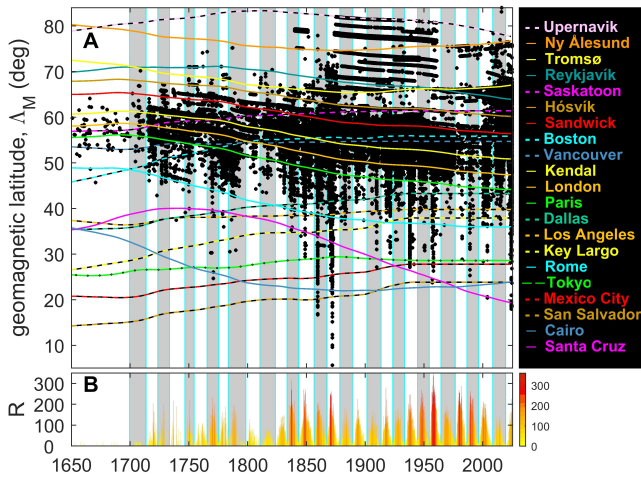
Figure 8. A A plot of the locations on a QD geomagnetic latitude ( \Lambda_M ) as a function of time for 194201 independent area-combined samples from 219244 observation records taken over the interval January 1650–July 2024. Vertical cyan lines mark sunspot minima and grey and white shading denotes, respectively, even- and odd-numbered sunspot cycles. The various coloured lines give the variation of \Lambda_M with time for several selected sites (named on the right-hand side), computed from the spline of gufm1 and IGRF geomagnetic field models. B Carrington rotation means of sunspot number, R shown in a bar-chart format where the histogram bars are coloured according to their height.
