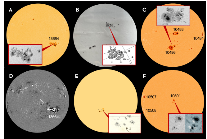
Figure 18. Active region sunspot groups associated with events ranked 1, 3, 4, 5, and 6 in Table 2. Sunspots groups are labelled with the AR numbers assigned by NOAA. A. Continuum image of the Solar disc made by the HMI (Helioseismic and Magnetic Imager) instrument on SDO (Solar Dynamics Observatory) on 10 May 2024 showing sunspot group 13664 (shown in greater detail in the inset); Part D , beneath A , shows the magnetogram taken simultaneously by the same instrument. B Richard Carrington's sunspot group drawings for 1 September 1859: the whole disk is from RAS MS Carrington 3, v. 2, f. 313a (reproduced courtesy the Royal Astronomical Society of London) and the close up detail is from his paper in Monthly Notices ( ). E. beneath B , shows a reconstruction of the sunspot group near the centre of the solar disc that is thought to have given rise to the storm of 4 February 1872: this is drawn from the solar drawings for 3 February by Angelo Secchi and Louis Bernaerts and contains only the common elements of those two drawings: the inset shows the sketch by Secchi (from Hayakawa et al. 2023c). C Continuum image of the Solar disc made by the MDI (Michelson Doppler Imager) instrument on SoHO (Solar and Heliospheric Observatory) satellite on 29 October 2003 showing sunspot group 10484 (shown in greater detail in the inset); Part F beneath C shows the solar disc 22 days later seen by the same instrument on 20 November 2003 with just one central group (10501): the inset shows the active region and a magnetogram plot, revealing the magnetic structure (Oreshina et al. 2012).
