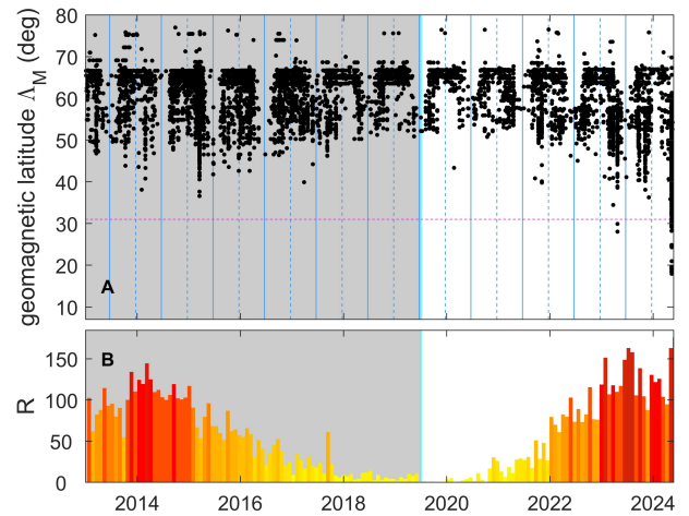
Figure 9. Same as Figure 8 but for the interval January 2013 to July 2024, covering approximately one solar cycle. In part A vertical solid and dashed blue lines have been added marking, respectively, the June and December solstices and a mauve horizontal dashed line marking the 31^\circ -threshold for an extreme event that is adopted here
