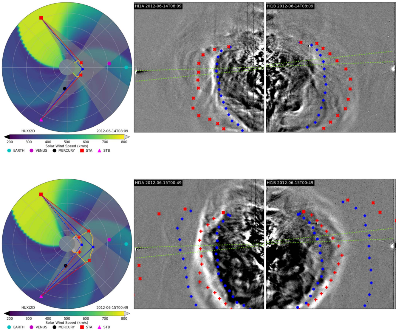
Figure 2. The left panels contain a snapshot of the solar wind speed on the equatorial plane as simulated with the HUXt model. The yellow and orange lines mark the boundaries of CME-1 and CME-2, respectively. The gray shaded areas show the fields of view of HI-A and HI-B. The middle and right panels show the observations of the same CME on the meridional plane from HI-A and HI-B. The dashed-green lines mark a 4^\circ position angle band around the solar equatorial plane. The red cross and red plus mark the flanks of the modeled CME-1 and CME-2. The blue diamonds mark the nose of CMEs. The flank and nose of the modeled CME-1 and CME-2 at each 5^\circ position angle are overlain on the HI images. An animation of this figure is available, showing the evolution of the two CMEs boundary by interacting with the ambient solar wind. It covers 25.3 hr starting at 01:29 on 2012 June 14. The realtime duration of the animation is 7 s.
