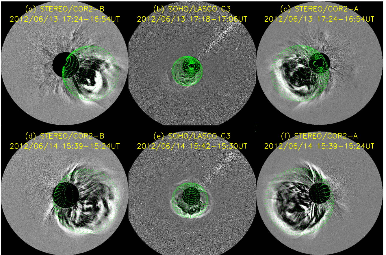
Figure 1. GCS fitting (green mesh) for each of the CMEs for contemporaneous images from SECCHI/COR2-B, SOHO/LASCO/C3, and SECCHI/COR2-A, from left to right, respectively. The panels show running difference images of CME-1 (top row) between 17:18 and 17:24 UT on 2012 June 13, and CME-2 (bottom row) between 15:39 and 15:42 UT on 2012 June 14.
