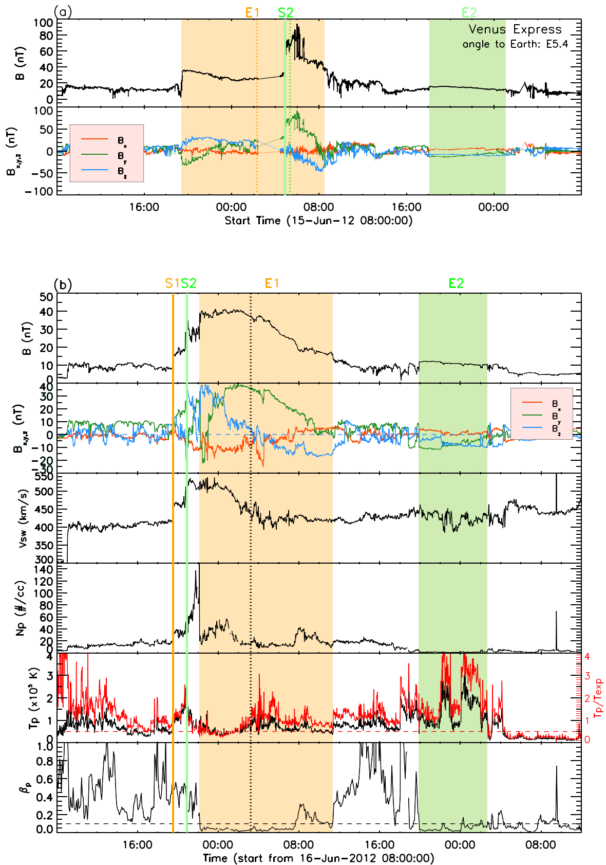
Figure 3. In situ observations of CME-1 and CME-2 at Venus and Earth. (a) VEX magnetic field strength and the x, y, and z components in VSO coordinates, (b) Wind in situ magnetic (x, y, and z components in GSE coordinates) and plasma data. The yellow and green shaded regions indicate the intervals of CME-1 and CME-2. The solid yellow and green vertical lines indicate the arrival of the shock driven by CME-1 and CME-2, respectively. The expected arrival times of CME-1 and CME-2 are indicated by vertical dashed lines (CME-1:yellow, CME-2:green).
