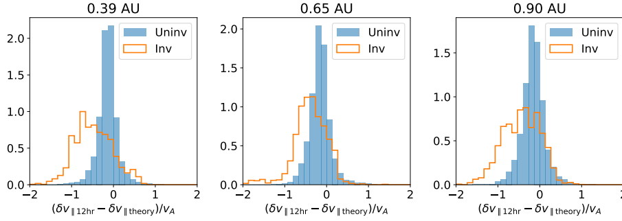
Figure 3. Histograms of the difference between \delta v_{\parallel} derived from the 12 hr average, and the theoretical value from Equation 2, \delta v_{\parallel\text{theory}} , for uninverted HMF (blue) and inverted HMF (orange) samples, for 3 heliocentric distances. \delta v_{\parallel\text{theory}} is computed using \sqrt{r_A} = [0.7, 0.6, 0.5] for the three distance bins, in order of increasing r . Histograms are normalised such that they integrate to unity.
