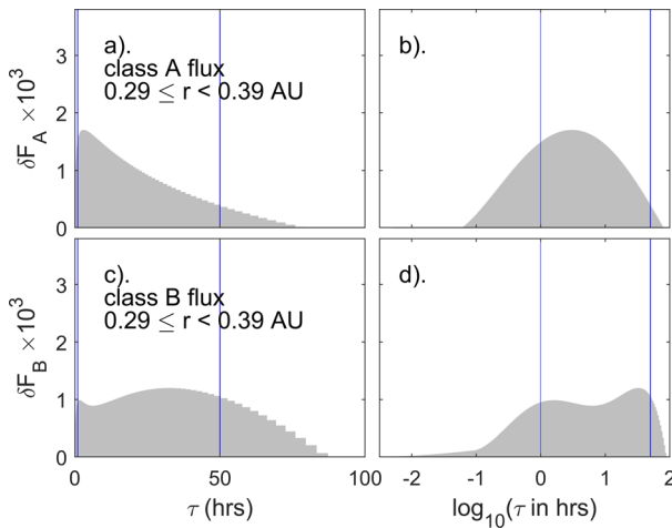
Figure 13 The same as Figures 10c and 10d for (top) Class-A flux and (bottom) Class-B flux observed by the Helios spacecraft at r < 0.39 AU, as defined by the pink and pale blue areas, respectively, in Figure 8b. In each panel, the area shaded grey gives the flux lost in increasing the averaging time between \tau_1 and \tau_2 [ \delta F ]; a and c show vertical bars of height \delta F between \tau_1 and \tau_2 and in b and d the bars are again of height \delta F but between \log_{10}(\tau_1) and \log_{10}(\tau_2) . Panels a and b are for Class-A OGH flux; c and d are for Class-B OGH flux. In each panel vertical blue lines are drawn for \tau = 1 hour and \tau = 50 hours for reference.
