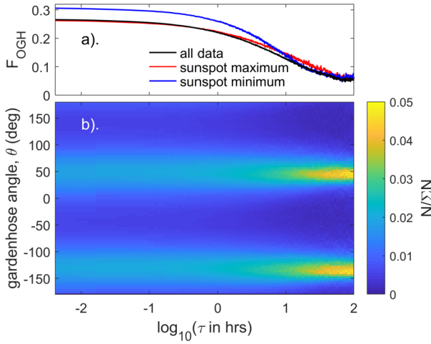
Figure 9 The effect of averaging on the distribution of gardenhose angle \theta for r = 1 AU. For timescales \tau \geq 1 minute ( \log_{10}(\tau \text{ in hours}) \geq 1.77 ) the data used are one-minute averages from the Omni dataset for 1996–2017. Plots are extended to \tau below one minute using 15-second averages of data from the ACE and Wind spacecraft for the same interval. Panel b shows N/\sum N (where N is counted in 4^\circ -wide bins of HMF gardenhose angle [ \theta ]) colour-coded as a function of \log_{10}(\tau \text{ in hours}) and \theta . Panel a shows the fraction [ F ] of the integrated total of the radial magnetic flux (toward or away) that is in a non-Parker-spiral Class-A or Class-B orientation (as defined by Figure 7a), as a function of \log_{10}(\tau \text{ in hours}) : the black line is for all years, the red line for three-year intervals around sunspot maxima, and the blue line for three-year intervals around sunspot minima.
