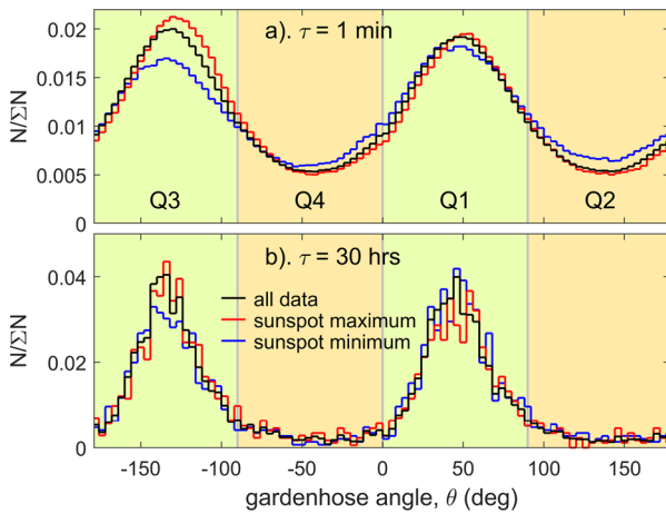
Figure 5 Occurrence distribution histograms as a function of observed gardenhose angle [ \theta ] for the near-continuous IMF data available for 1996 to 2017 (inclusive): the black lines are for all data, red lines for the six years within one year of one of the two sunspot maxima, and the blue lines are for the six years within one year of a sunspot minimum (which is here taken to include 2017). The number [ N ] of valid samples in 4^\circ -wide bins of \theta are counted and normalised to the sum for all 90 bins [ \sum N ]. (a) is for an averaging timescale \tau = 1 minute, and (b) is for \tau = 30 hours. As in Figures 1 and 2, OGH and GH sectors are shaded orange and green , respectively. The four quadrants are labelled Q1 (T-field in gardenhose orientation), Q2 (A-field in ortho-gardenhose orientation), Q3 (A-field in gardenhose orientation), and Q4 (T-field in ortho-gardenhose orientation), where T and A are “Toward” and “Away” from the Sun, respectively ( B_X \geq 0 and B_X < 0 ).
