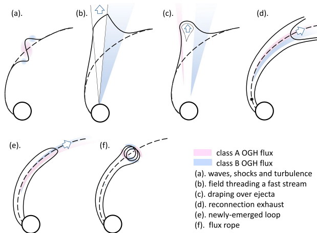
Figure 4 Schematics of some of the dynamical causes of OGH HMF orientations in near-Earth interplanetary space. The areas shaded pink and pale blue are snapshots of where Class-A and Class-B OGH flux (see Figure 3) exist at a given time and hence in cases d and e , their radial extent depends on how long the reconnection and new loop emergence (respectively) persist. The dashed lines are an undisturbed Parker-spiral HMF field-line orientation.
