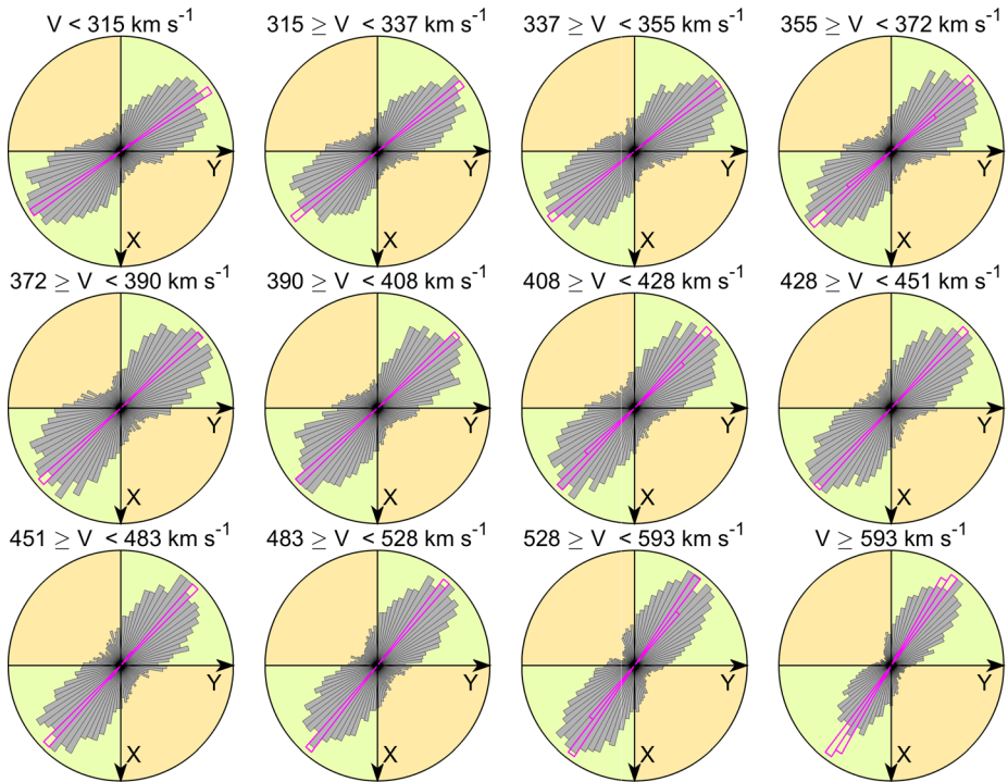
Figure 1 Occurrence distribution of near-Earth heliospheric field (HMF) orientation. The grey polar histograms show the distributions of the observed field gardenhose angle \theta (computed using Equation 1) in the GSE X – Y frame from 1-hour averages ( \tau = 1 hour) of the HMF components for the years 1996–2017 (inclusive, giving 161,620 valid samples). The data are divided into twelve bins of equal sample numbers (13,468 in each) between the percentiles of the distribution of the radial solar-wind speeds [V] , which are 315, 337, 355, 372, 390, 408, 428, 451, 483, 528 and 593 \text{km s}^{-1} . The mauve histograms show the corresponding distributions of the orientation predicted from Parker-spiral theory ( \theta_p , computed using Equation 4) for the hourly mean observed radial solar-wind speed V . The rotation of the means and modes of the observed gardenhose distribution towards the X axis with increasing V matches well that in the predicted field orientation. The ortho-gardenhose (OGH) and gardenhose (GH) sectors are shaded orange and green, respectively. The toward the Sun (T) OGH field is in the positive Y , positive X sector and the away from the Sun (A) OGH field is the negative Y , negative X sector and both are seen in all velocity ranges being most common for the lowest V and less common for the highest V .
