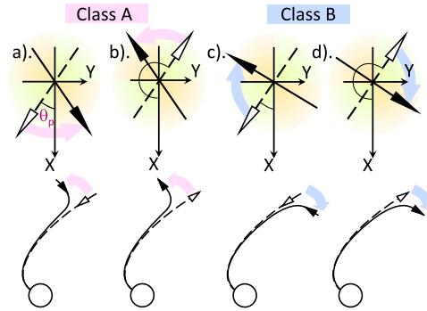
Figure 3 Schematic of \theta , sectors and HMF deviations from Parker-spiral. The top panels show are local views of the near-Earth ecliptic plane from the North ( i.e. looking in the -Z GSE direction): as in Figure 1, the OGH and GH quadrants are shaded orange and green, respectively. The lower panels are views of the inner heliosphere looking down from over the North Pole of the Sun. In both cases, OGH field is shown by solid arrows with open and dashed arrows giving the ideal Parker-spiral field direction. Parts a and b are termed Class-A deflections of the local IMF vector from the Parker-spiral with anticlockwise rotation of the near-Earth field vector when viewed in the -Z -direction (pink arrows); parts c and d are termed Class-B deflections from the Parker-spiral with clockwise rotation of the field vector when viewed in the -Z -direction (pale blue arrows). Note that in the lower panels the arrows show the displacement of the HMF field lines from the Parker spiral, not the sense of rotation.
