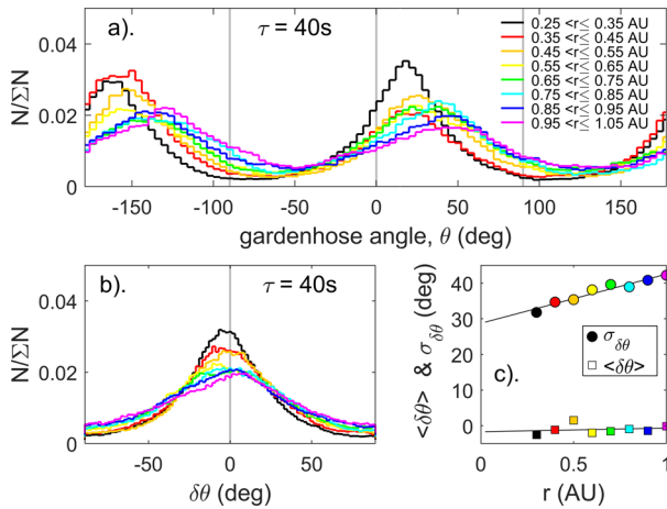
Figure 6 Helios-1 and Helios-2 data showing how the gardenhose-angle distribution varies between 0.3 and 1 AU. Data are sorted into eight non-overlapping bins of heliocentric distance [ r ] that are 0.1 AU wide and centred on [0.3:0.1:1.0] AU. (a) Histograms of the normalised number of samples in bins of gardenhose angle \theta that are 4^\circ wide [ N/\sum N ] colour-coded by the range of r using the key given. (b) The distributions of the deviations from the predicted Parker-spiral angle \delta\theta for the same ranges of r and using the same colour scheme. (c) The variations with r of the means and standard deviations of the \delta\theta distributions shown in (b) [respectively \langle\delta\theta\rangle and \sigma_{\delta\theta} ]. The black lines are the best least-squares linear regression fits.
