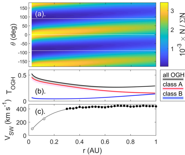
Figure 7 (a) Model of the evolution of the distributions of gardenhose angle \theta with heliocentric distance r using Gaussian distributions of the deviations from the Parker-spiral direction of mean \langle \delta\theta \rangle and standard deviation \sigma_{\delta\theta} given by the regression fits in Figure 6c. The total toward and away distributions are assumed to be symmetrical and the linear variations in \langle \delta\theta \rangle and \sigma_{\delta\theta} seen at r > 0.3 are extrapolated to closer to the Sun. The Parker-spiral direction at each r is evaluated using the velocity variation [V(r)] shown in Panel c, which is a fifth-order polynomial fit to the observed average velocities in the Helios data (solid circles) and values at r of 6 R_{\odot} and 26 R_{\odot} (open circles) derived by applying Fourier motion filters to SOHO/LASCO-C3 movies observed from 1999 to 2010 by Cho et al. (2018). Panel b shows the predicted fraction of time that the field is in an OGH orientation, T_{OGH} : the black line is for all field, the red line for Class-A OGH field, and the blue line for Class-B OGH field (see Figure 2). The areas shaded grey, pink, and pale blue around the black, red, and blue lines are the uncertainties introduced by the uncertainty in \langle \delta\theta \rangle .
