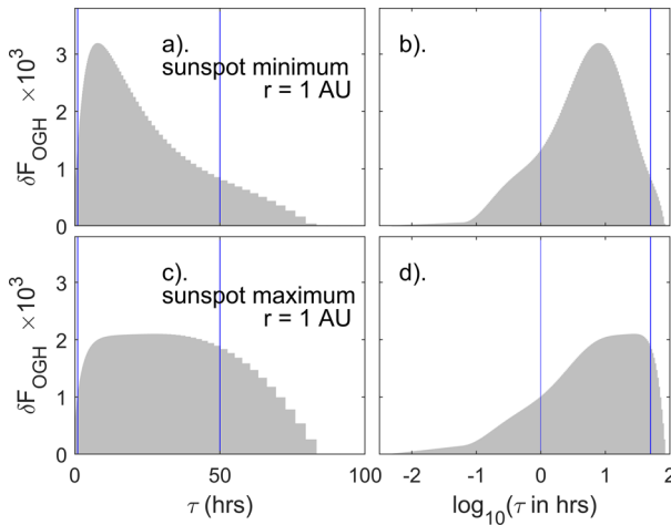
Figure 11 The same as Figures 10c and 10d for (top) data at r = 1 AU within one year of sunspot minimum and (bottom) one year of sunspot maximum. In each panel, the area shaded grey gives the flux lost in increasing the averaging time between \tau_1 and \tau_2 [ \delta F ]: a and c show vertical bars of height \delta F between \tau_1 and \tau_2 and in b and d the bars are again of height \delta F but between \log_{10}(\tau_1) and \log_{10}(\tau_2) . Panels a and b are for observations in a three-year interval around sunspot minimum (the years 1996, 1997, 2007, 2008, 2009, and 2017); c and d are for observations in a three-year interval around the sunspot maxima (the years 2000, 2001, 2002, 2012, 2013, and 2014). In each panel vertical blue lines are drawn for \tau = 1 hour and \tau = 50 hours for reference.
