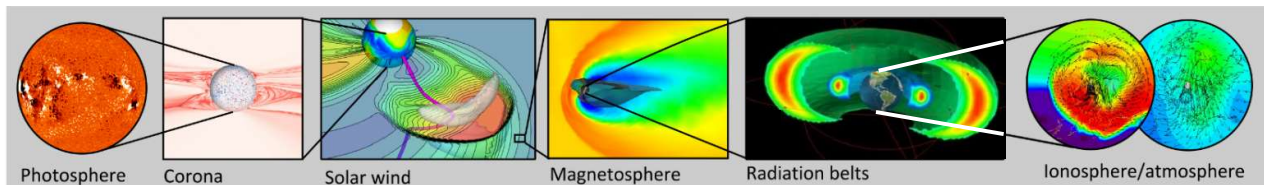
2. Illustration of the number of different numerical models that would be involved in a full “cradle-to-grave” numerical space weather forecast scheme that starts with observations of the solar photosphere. This poses many problems in terms of spatial and temporal scale-changing when daisy-chaining the models together (adapted from Owens et al. 2014). The main area missing from UK capabilities has been a numerical MHD model of the magnetosphere, but this is now being addressed at Imperial College by adapting the GORGON model, originally developed for studies of laboratory plasmas (Mejnertsen et al. 2018).
