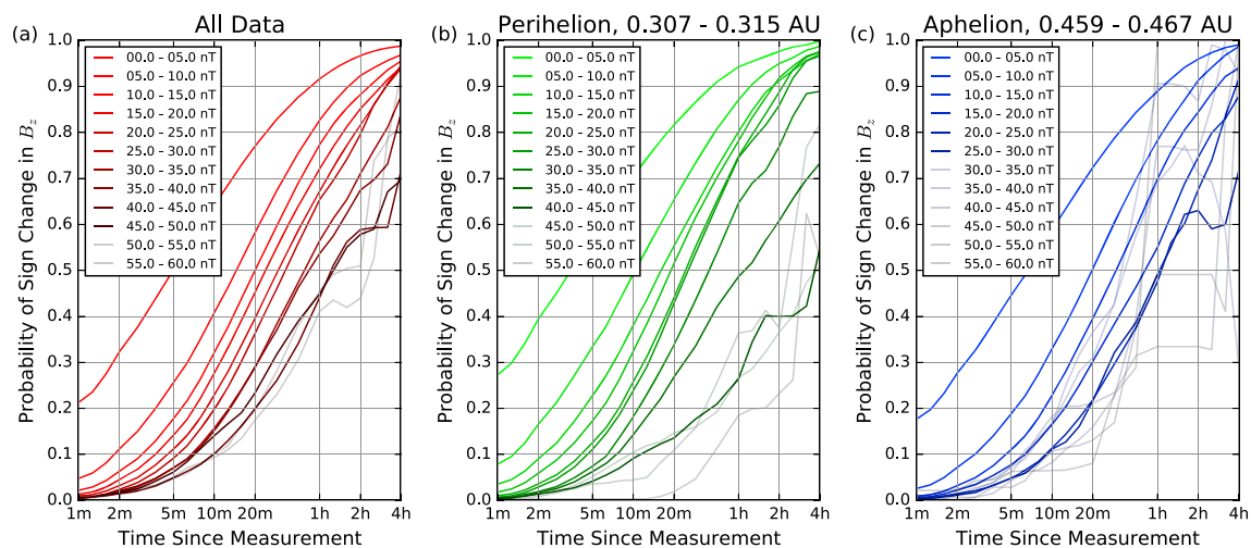
Figure 8. Probabilities of a change in polarity of the z component of the IMF for the following: (a) all data, (b) near perihelion, and (c) near aphelion as a function of time. Each different line represents the probability of a sign change occurring for an initial IMF magnitude within one of the 5 nT bins listed in the legend of each panel. Some lines with higher starting IMF magnitudes are grayed out in each plot as there are not enough instances of such field strengths to create a reliable probability function.
