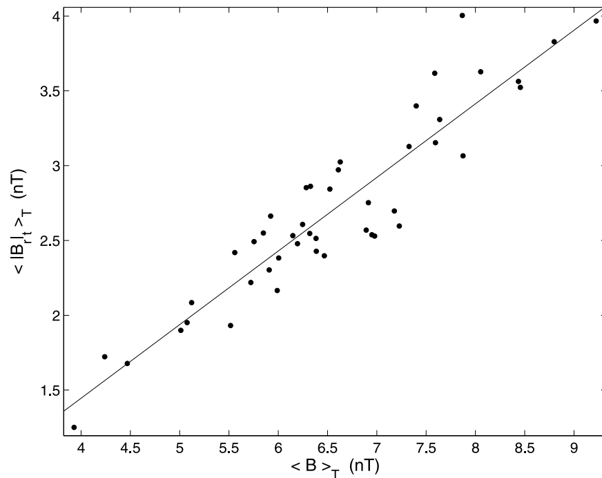
Figure 3. Scatterplot of the mean of the modulus of the radial IMF, \langle |B_r|_{t} \rangle_T as a function of IMF magnitude \langle B \rangle_T for the OMNI2 data set for 1963–2010. The preaveraging timescale (on which the modulus is taken) is t = 1 day, and the final averaging timescale is T = 1 year. Only means for years with >25\% data availability are included in the plot and the regression. The correlation coefficient is r = 0.93 (significance level 99.88%), and the ordinary best fit linear regression fit shown has a slope d = 0.492 \pm 0.029 and an intercept e = -0.522 \pm 0.136 .
