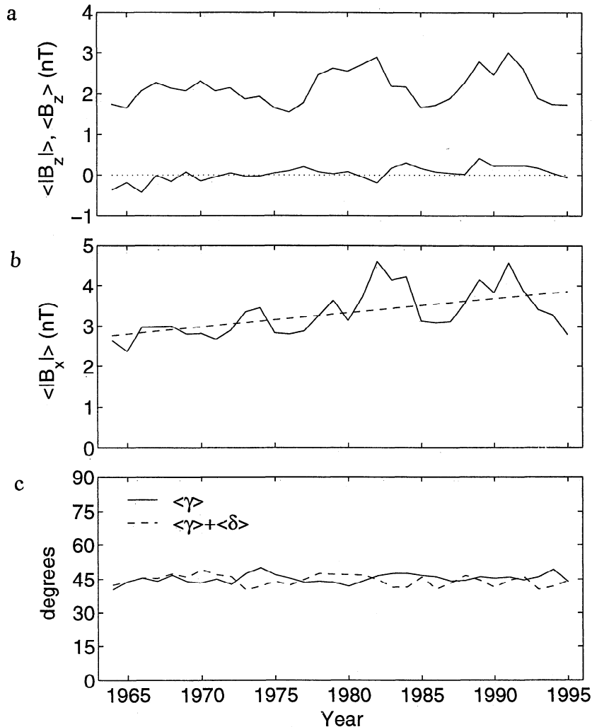
Figure 11. Annual means of the IMF seen at r = 1 AU in GSE coordinates: (a) \langle B_z \rangle (which is always close to zero) and \langle |B_z| \rangle . (b) \langle |B_x| \rangle = |B_r| . (c) The mean of the IMF garden-hose angle in the X-Y GSE frame: predicted from Parker spiral theory \langle \gamma \rangle (solid line) and observed \langle \gamma \rangle + \langle \delta \rangle (dashed line).
