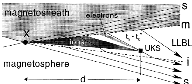
Figure 2. Schematic of AMPTE-UKS in the open LLBL, between the magnetopause (m) and interior (i) Alfvén waves emanating from the reconnection site (X-line), X. Field lines evolving away from X are shown at five elapsed times since they were opened ( t_s - t_0 ), including zero for the magnetic separatrices (s). The spectrum of sheath ions reaching UKS has a spread of trajectories shown by the dark shaded wedge, the trajectories of the sheath electrons are much closer to field-aligned (lighter shaded wedge). The populations seen depend on UKS's depth into the LLBL, i.e. on the ( t_s - t_0 ) at a given distance d from X.
