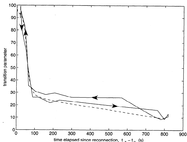
Figure 4. Solid line: hodogram showing the variation of the observed transition parameter \tau with the time-elapsed since reconnection ( t_s - t_0 ), from the fit to the ion data shown in figure 3. Dashed line: model prediction made by applying the transition parameter to the modelled electron data shown in figure 6.
