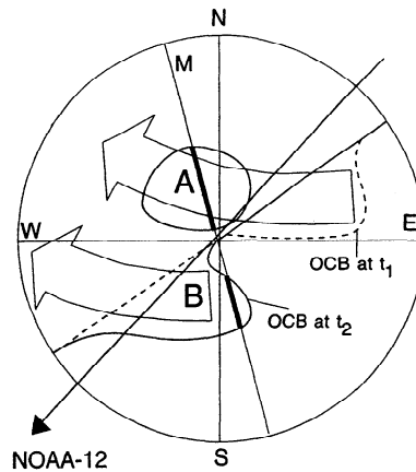
Figure 5. A schematic illustration summarizing the observations. The pair of westward moving auroral events, A and B, were both observed by the photometer scanning along the magnetic meridian M, but were produced by active X-line segments, respectively, to the east and to the west that meridian. The open-closed boundary (OCB) is shown at times just after the two reconnection pulses by dashed and solid lines, respectively: for the events shown in Figure 2 t_1 is near 0945 and t_2 is about 0946 UT. The OCB is slightly equatorward of the LLBL/CPS boundary identified to border on the equatorward edge of the 630.0 nm aurora.
