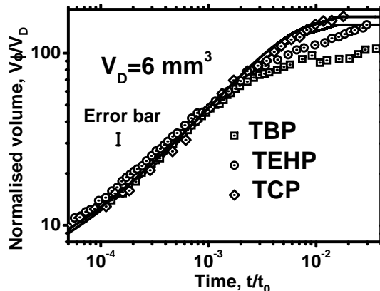
FIG. 15. Spreading of TCP, TEHP and TBP liquid drops ( V_D = 6 mm 3 ) in R = 0.25 mm sand ( R = 0.26 mm for TCP liquid). Comparison between experimental data and simulations using superfast diffusion model (28) with initial distribution of saturation given by (31). Normalised wet volume V_\phi/V_D (inverse average saturation \bar{s}^{-1} ) as a function of the reduced time t/t_0 , t_0 = L_0^2/D_f . Experimental data are shown by symbols and simulations are presented by the solid lines. Parameters of the simulations and the fitting are summarized in Table I.
