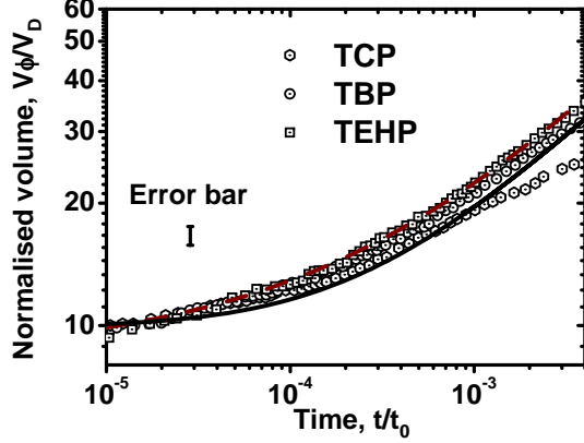
FIG. 17. Spreading TCP, TEHP and TBP liquid drops ( V_D = 3 \text{ mm}^3 ) in sands with R = 0.25 \text{ mm} in one-dimensional geometry. Comparison between experimental data and simulations using superfast diffusion model (28) with initial distribution of saturation given by (33). Normalised wet volume V\phi/V_D (inverse average saturation \bar{s}^{-1} ) as a function of the reduced time t/t_0 , t_0 = L_0^2/D_f . Experimental data are shown by symbols and simulation is presented by the solid line. Parameters of the simulations and the fitting are summarized in Table I. The dashed line (brown) is the fit V\phi/V_D = A + B(t/t_0)^{0.5} at A \approx 8.5 and B \approx 440 .
