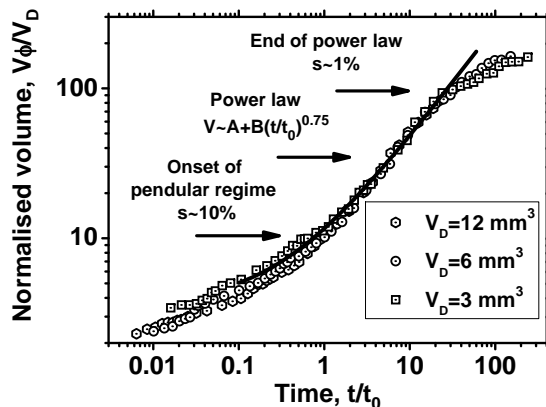
FIG. 5. Spreading of TCP liquid drops of different volumes V_D = 3, 6 and 12 \text{ mm}^3 in R \approx 0.26 mm sand in a three-dimensional case. Normalized volume V\phi/V_D (inverse average saturation \bar{s}^{-1} ) as a function of reduced time t/t_0 , where t_0 = \frac{V_D^{2/3}}{D_e} , D_e = 1.85 \times 10^{-10} \text{ m}^2/\text{s} ( t_0 \approx 300 min at V_D = 6 \text{ mm}^3 ). The solid line is the fit V\phi/V_D = A + B(t/t_0)^{0.75} at A = 3.6 and B = 8 .
