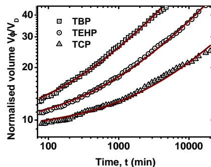
FIG. 7. Spreading of TCP, TEHP and TBP liquid drops ( V_D = 3 \text{ mm}^3 ) in R \approx 0.25 mm sand in the channels, as in Fig. 6. Normalised wet volume V\phi/V_D (inverse average saturation \bar{s}^{-1} ) as a function of time. The experimental data are shown by symbols and the solid lines (brown) are the fits V\phi/V_D = A + Bt^{0.5} .
