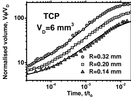
FIG. 16. Spreading TCP liquid drops ( V_D = 6 \text{ mm}^3 ) in sands with different grain radii R = 0.14, 0.20 and 0.32 \text{ mm} . Comparison between experimental data and simulations using superfast diffusion model (28) with initial distribution of saturation given by (31). Normalised wet volume V\phi/V_D (inverse average saturation \bar{s}^{-1} ) as a function of the reduced time t/t_0 , t_0 = L_0^2/D_f . Experimental data are shown by symbols and simulations are presented by solid lines. Parameters of the simulations and the fitting are summarized in Table I.
