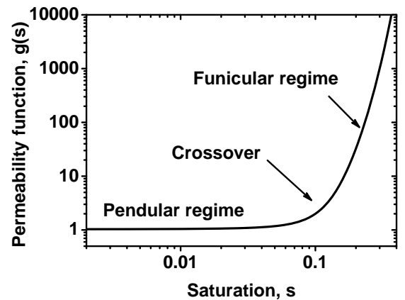
FIG. 11. Permeability function g(s) versus saturation s at \alpha_g = 16.5 , \beta_g = 1.65 and f_0 = 1 .
