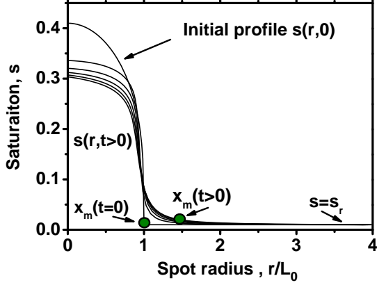
FIG. 20. Simulation of spreading of TEHP liquid drops ( V_D = 6 \text{ mm}^3 ) in pre-wetted sands with the background saturations level s_r = 1\% using the augmented model (28) with initial conditions (34) at s_a = 0.4 , r_a = 4 and \lambda_a = 0.3 with s_0^e \approx 0.0068 .
