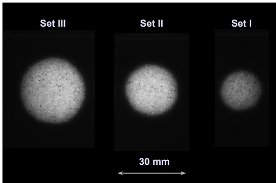
FIG. 4. UV fluorescence images of wet areas taken after \approx 45000 min of spreading from above the sand bed prepared using R \approx 0.26 mm sand. From left to right the image is for the sets III, II and I, as in Table I.
