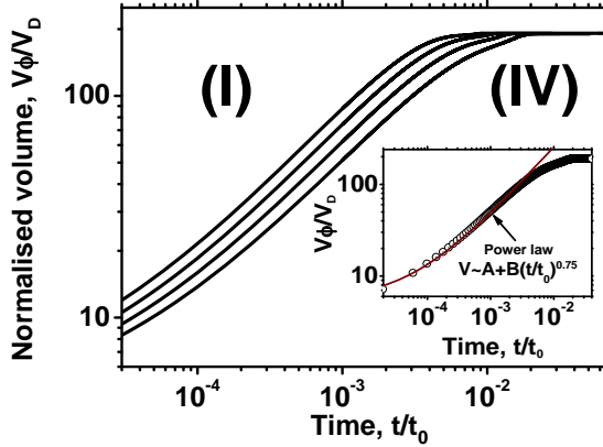
FIG. 12. Simulation of spreading in a three-dimensional spherically symmetric case using augmented superfast diffusion model (28) with initial distribution (31) at \lambda_a = 0.3 , s_a = 0.4 , \alpha_g = 16.5 , \beta_g = 1.65 , f_0 = 1 and s_f = 0.0052 , but at different values of parameter s_f - s_0^e . Normalised wet volume V\phi/V_D (inverse average saturation \bar{s}^{-1} , solid lines) as a function of the reduced time t/t_0 , t_0 = L_0^2/D_0^e . From left to right: (I) s_f - s_0^e = 0.0001 , (II) s_f - s_0^e = 0.0002 , (III) s_f - s_0^e = 0.0004 , (IV) s_f - s_0^e = 0.0008 . Insert shows the power law V\phi/V_D = A + B(t/t_0)^{0.75} (solid line, brown) in comparison with the numerical data (symbols, black) at s_f - s_0^e = 0.0008 .
