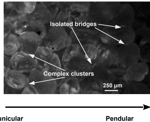
FIG. 3. An UV fluorescence image of the dyed liquid (TEHP) distribution (the bright areas) in sands in the transition from the funicular to the pendular regimes of wetting, at s > 10\% .
