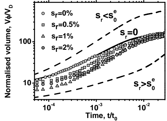
FIG. 19. Spreading of TEHP liquid drops ( V_D = 6 \text{ mm}^3 ) in pre-wetted sands with different background saturations levels s_r = 0, 0.5, 1 and 2\% . Normalised wet volume V\phi/V_D (inverse average saturation \bar{s}^{-1} ) as a function of the reduced time t/t_0 , t_0 = L_0^2/D_f . The experimental results are shown by symbols. The results of numerical simulations are shown by solid lines ( s_r = 0\% ) and by dashed lines s_r = 1\% and s_r = 0.5\% .
