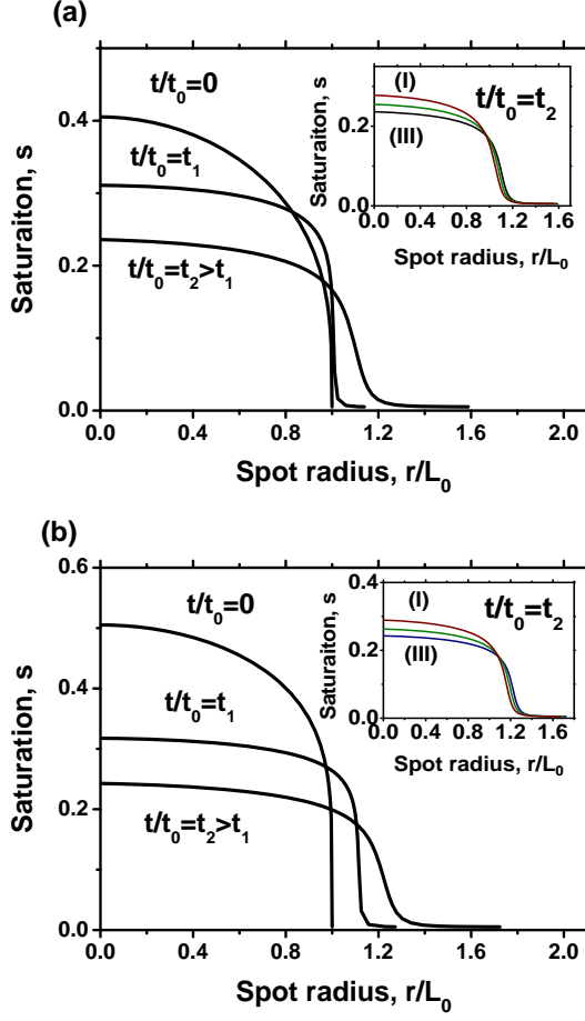
FIG. 13. Simulation of spreading in a three-dimensional spherically symmetric case using augmented superfast diffusion model (28) at different initial distributions (31). Saturation s(r, t) as a function of the reduced spot radius r/L_0 at t/t_0 = 0 , t/t_0 = t_1 = 3 \times 10^{-6} and t/t_0 = t_2 = 6 \times 10^{-5} at fixed values of \alpha_g = 16.5 , \beta_g = 1.65 , f_0 = 1 , s_f = 0.0052 and s_f - s_0^e = 0.0002 . (a) \lambda_a = 0.3 and s_a = 0.4 ; (b) \lambda_a = 0.2 and s_a = 0.5 . The inserts show variation of the saturation profile at t = t_2 with the parameters of the augmenting function g(s) . Here (I) \alpha_g = 12.5 and \beta_g = 1.25 , (II) \alpha_g = 14.5 and \beta_g = 1.45 , and (III) \alpha_g = 16.5 and \beta_g = 1.65 .
