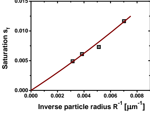
FIG. 10. Saturation s_f as a function of R^{-1} shown by symbols. The solid line is the fit s_f = A_f R^{-1} + B_f R^{-2} at A_f = 1.5 \mu\text{m} and B_f = 29 \mu\text{m}^2 .
